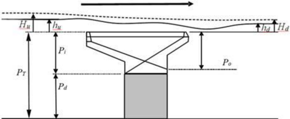
Figure 7: Cross section of the physical parameters nomenclature
